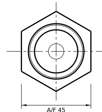
VIEW FROM ROD END (SCALE 1:1.5)
