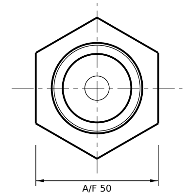
VIEW FROM ROD END (SCALE 1:1.5)
