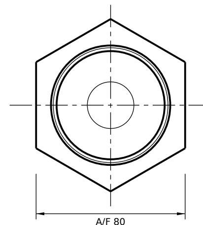
VIEW FROM ROD END (SCALE 1:2)
