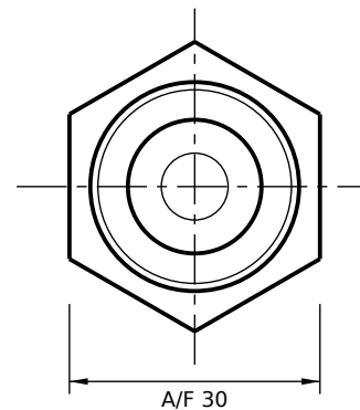
VIEW FROM ROD END (SCALE 1:1)
