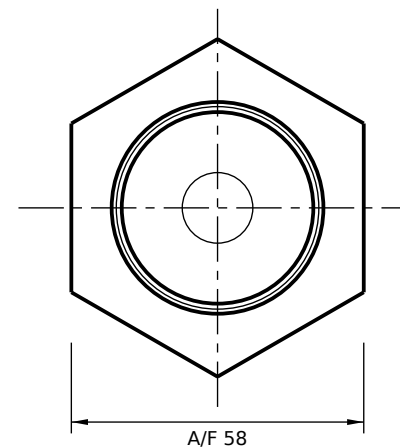
VIEW FROM ROD END (SCALE 1:1.5)
