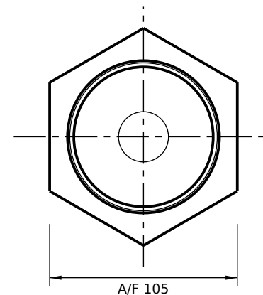
VIEW FROM ROD END (SCALE 1:3)
