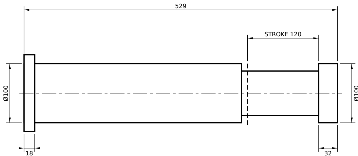
REAR FLANGE MOUNT (RS)
