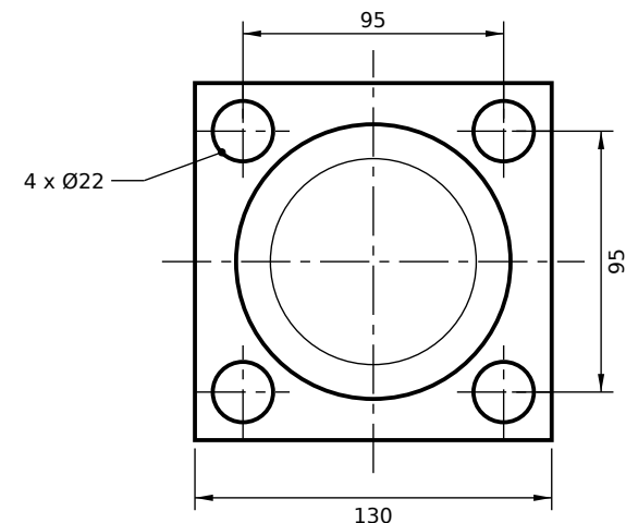
VIEW FROM ROD END (SCALE 1:3)
