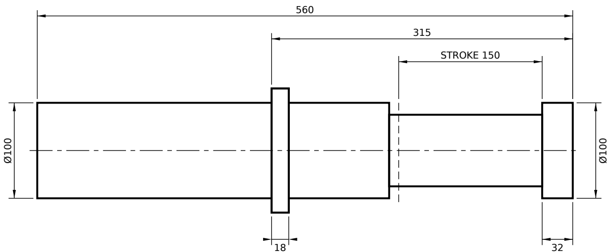
FRONT FLANGE MOUNT (FS)
