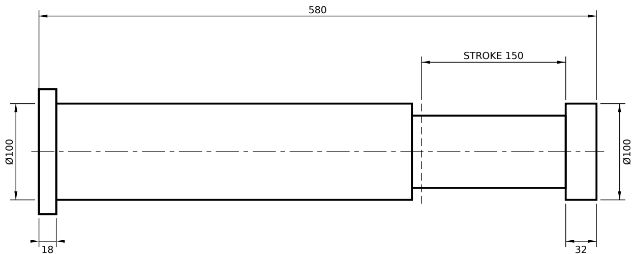
REAR FLANGE MOUNT (RS)
