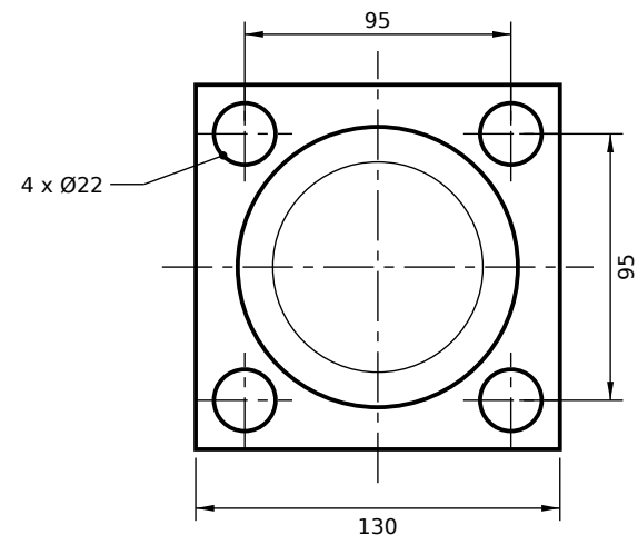
VIEW FROM ROD END (SCALE 1:3)
