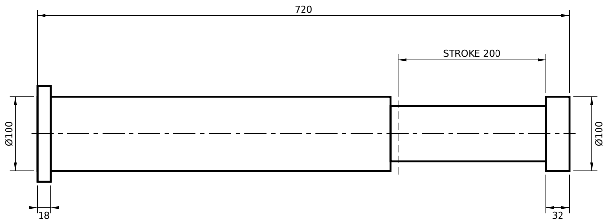
REAR FLANGE MOUNT (RS)
