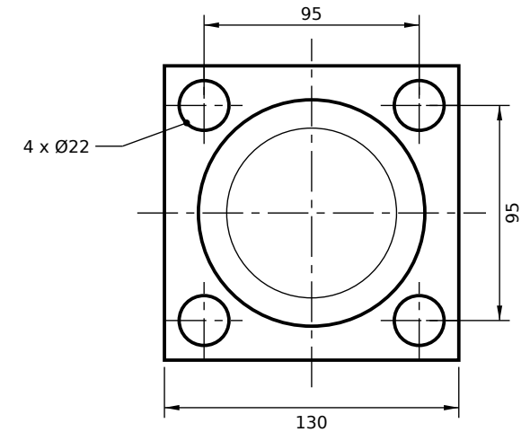
VIEW FROM ROD END (SCALE 1:3)
