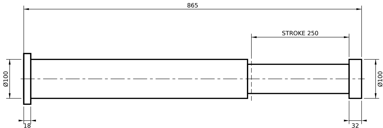
REAR FLANGE MOUNT (RS)
