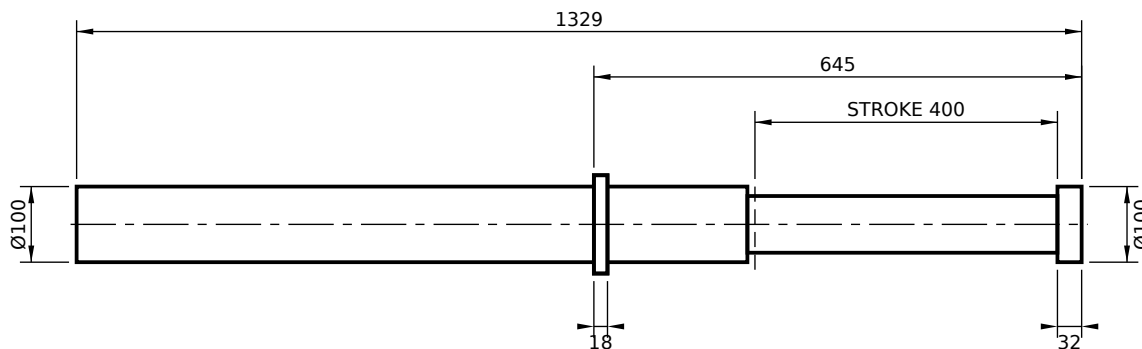
FRONT FLANGE MOUNT (FS)
