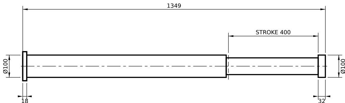
REAR FLANGE MOUNT (RS)
