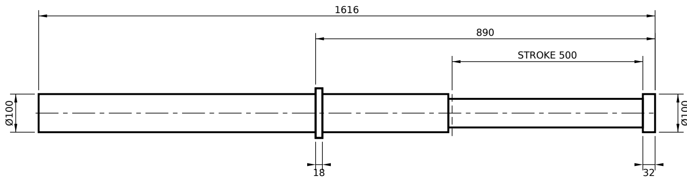
FRONT FLANGE MOUNT (FS)
