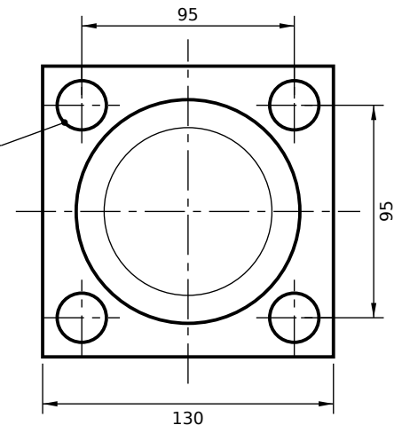
VIEW FROM ROD END (SCALE 1:3)
