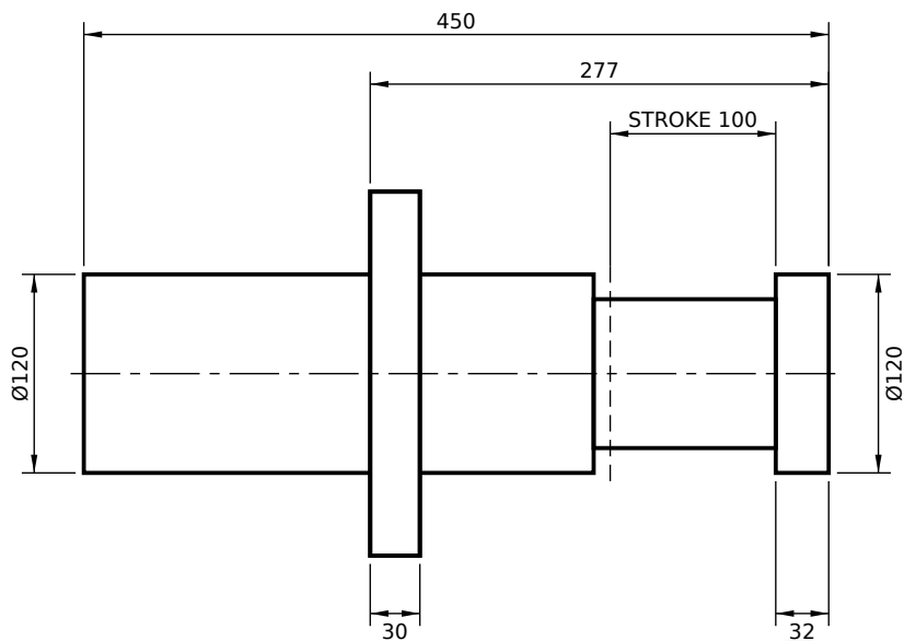
FRONT FLANGE MOUNT (FS)
