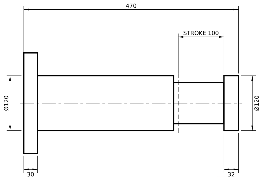
REAR FLANGE MOUNT (RS)
