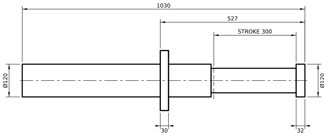
FRONT FLANGE MOUNT (FS)
