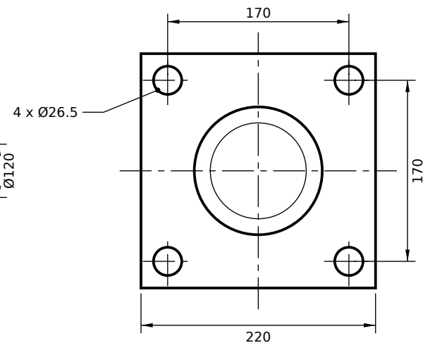
VIEW FROM ROD END (SCALE 1:5)
