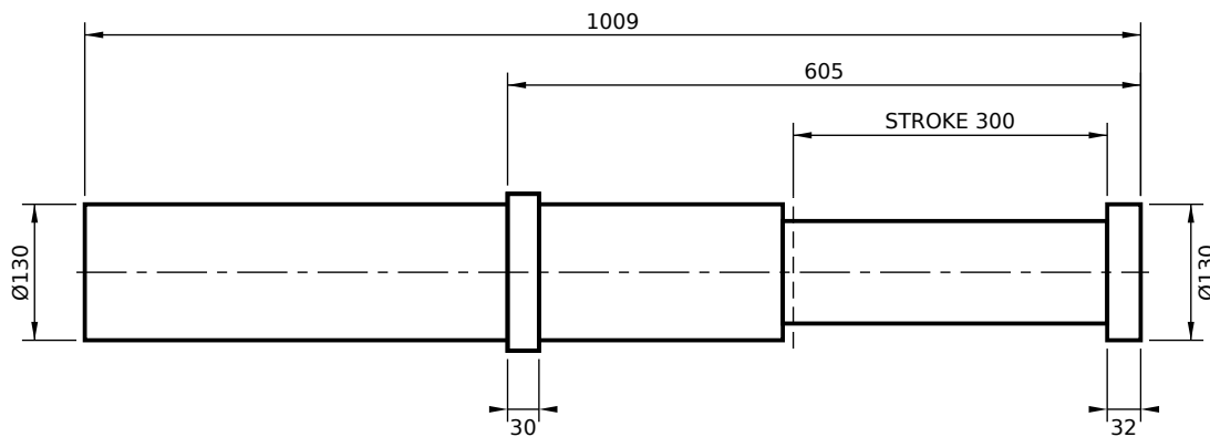
FRONT FLANGE MOUNT (FS)
