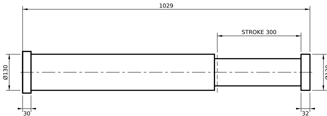
REAR FLANGE MOUNT (RS)
