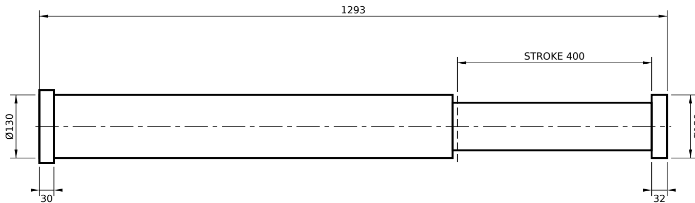
REAR FLANGE MOUNT (RS)
