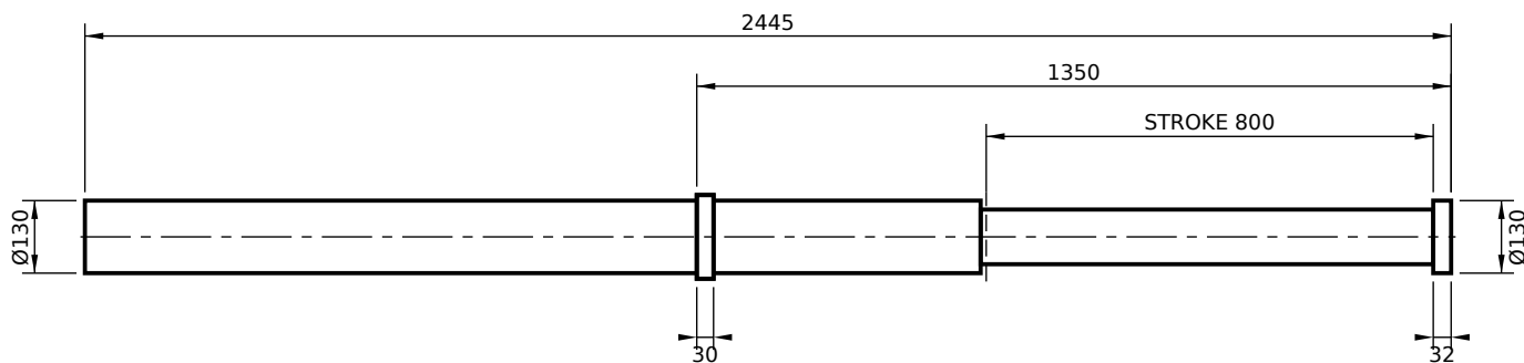
FRONT FLANGE MOUNT (FS)
