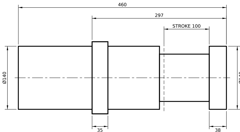
FRONT FLANGE MOUNT (FS)
