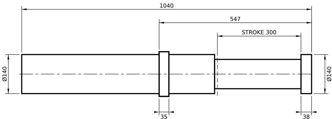
FRONT FLANGE MOUNT (FS)
