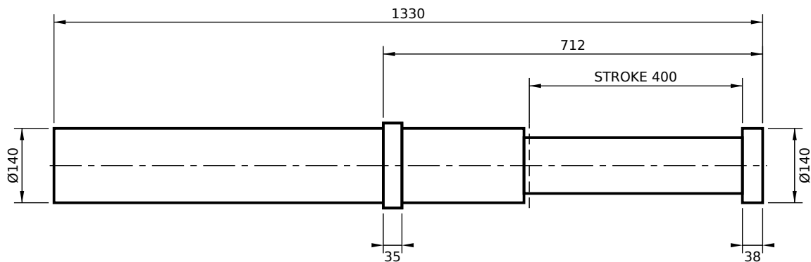
FRONT FLANGE MOUNT (FS)
