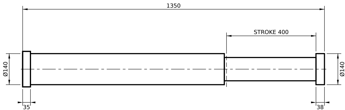
REAR FLANGE MOUNT (RS)
