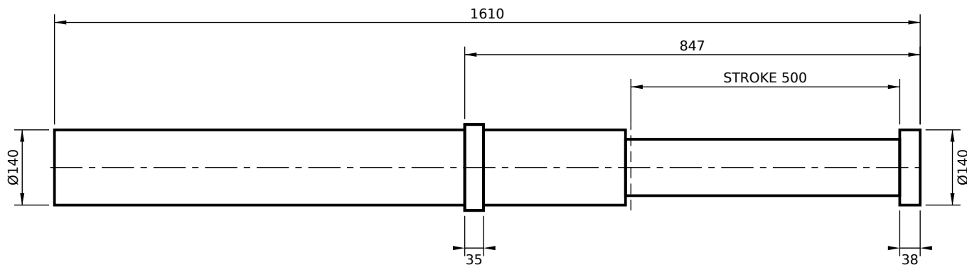
FRONT FLANGE MOUNT (FS)
