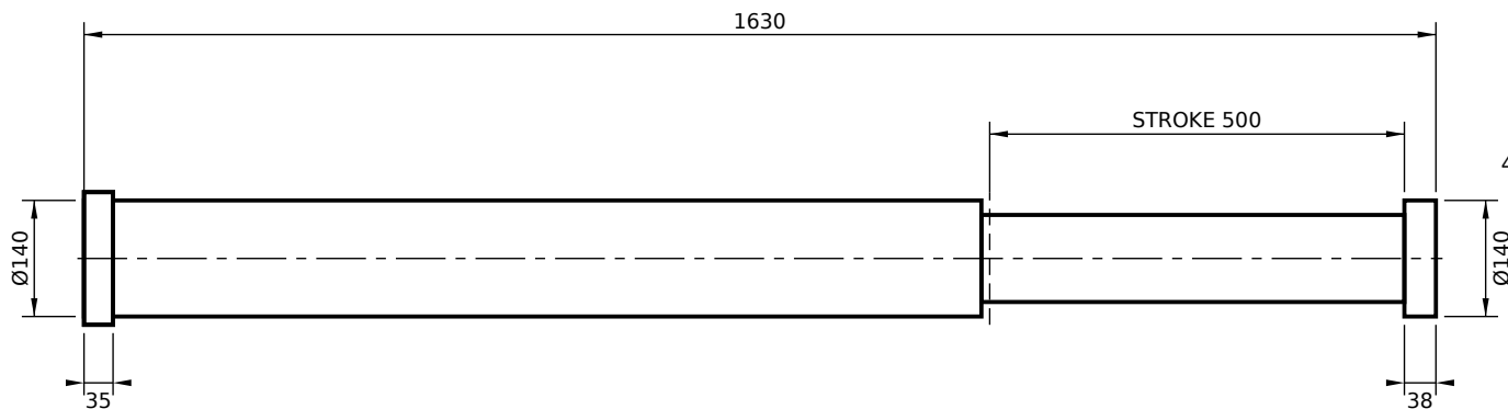
REAR FLANGE MOUNT (RS)
