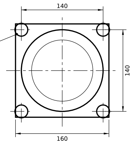
VIEW FROM ROD END (SCALE 1:4)
