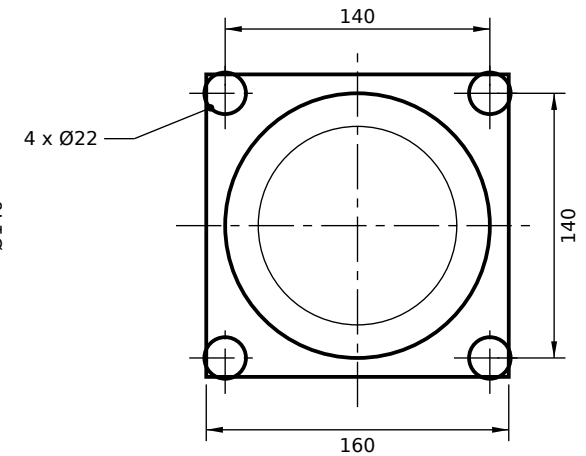
VIEW FROM ROD END (SCALE 1:4)
