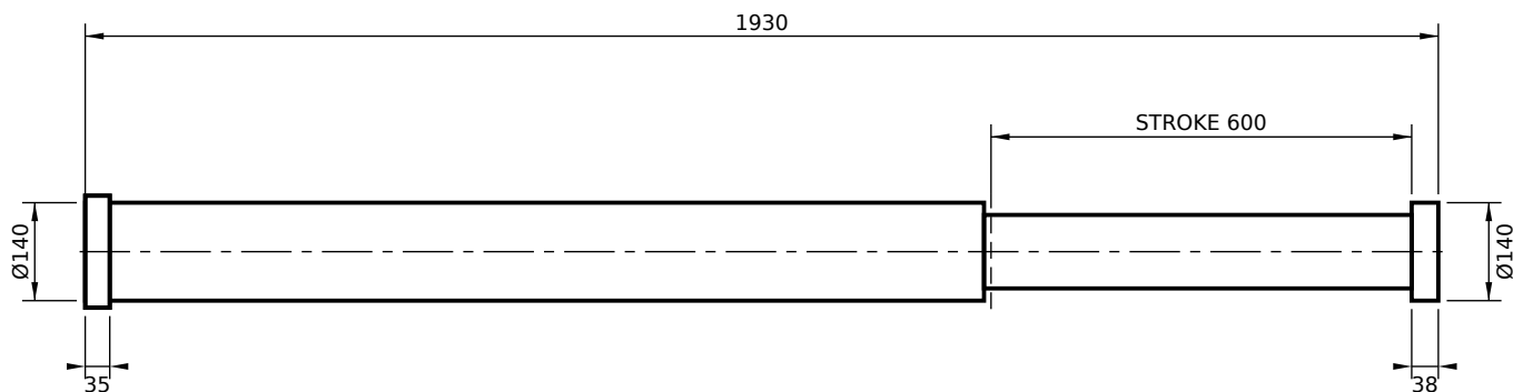
REAR FLANGE MOUNT (RS)
