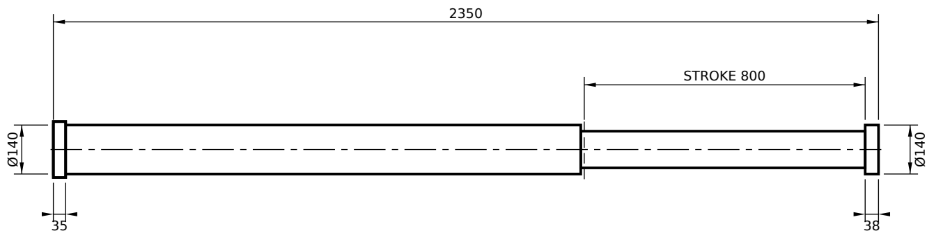
REAR FLANGE MOUNT (RS)
