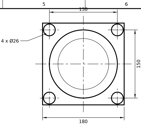
VIEW FROM ROD END (SCALE 1:4)
