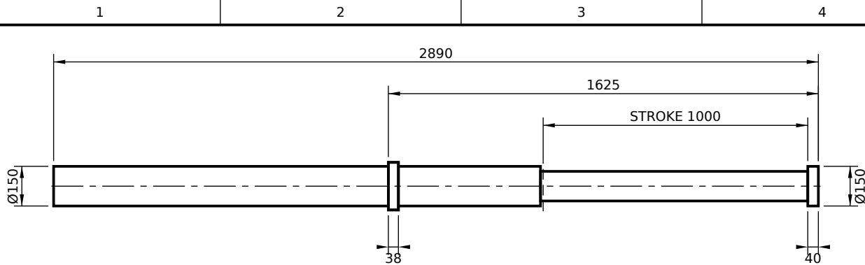
FRONT FLANGE MOUNT (FS)
