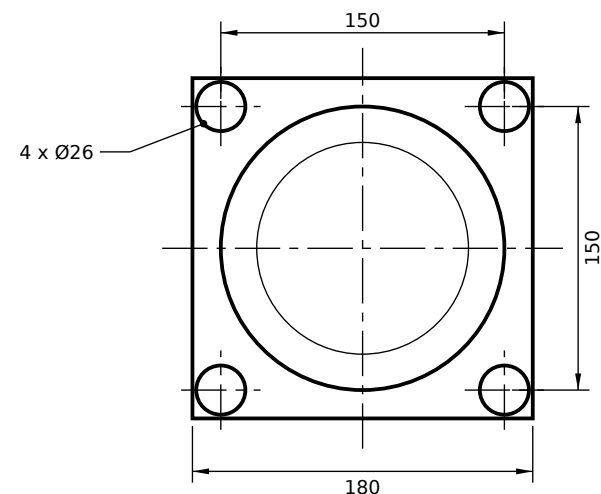
VIEW FROM ROD END (SCALE 1:4)
