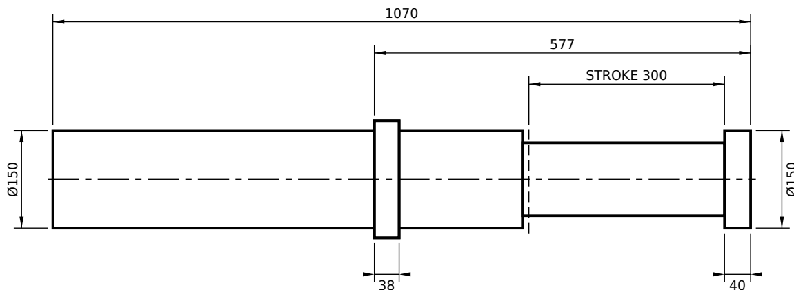
FRONT FLANGE MOUNT (FS)
