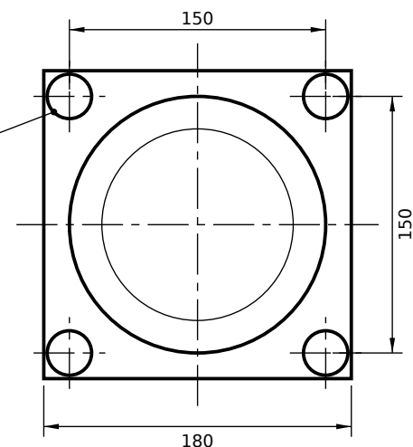
VIEW FROM ROD END (SCALE 1:4)
