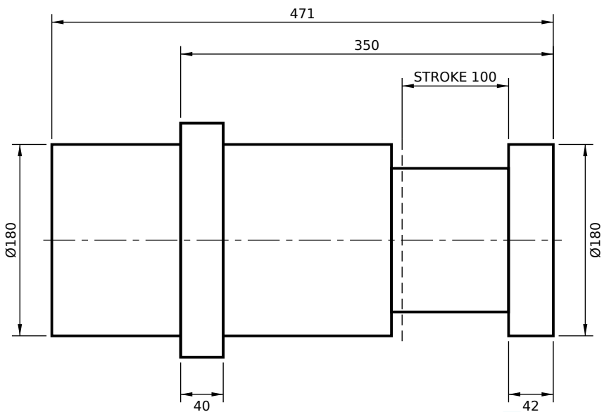
FRONT FLANGE MOUNT (FS)
