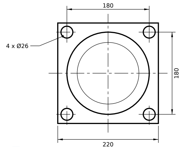
VIEW FROM ROD END
