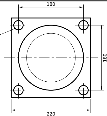
VIEW FROM ROD END (SCALE 1:5)
