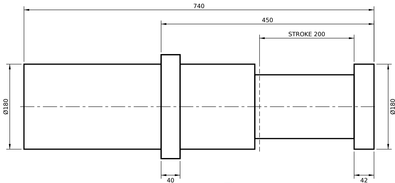
FRONT FLANGE MOUNT (FS)
