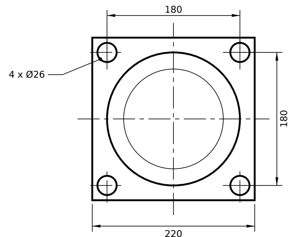
VIEW FROM ROD END (SCALE 1:5)
