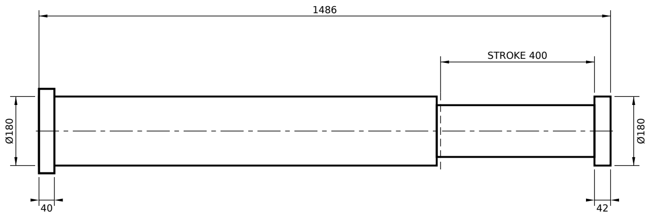
REAR FLANGE MOUNT (RS)
