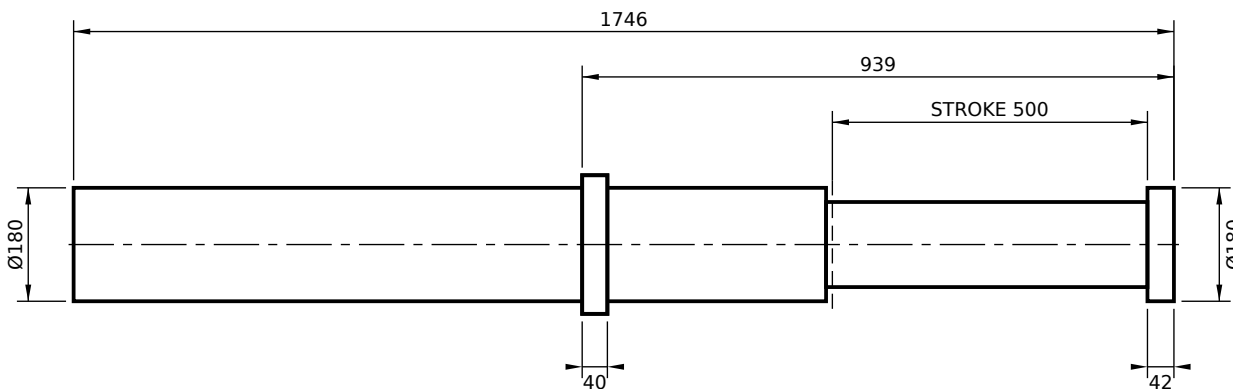
FRONT FLANGE MOUNT (FS)
