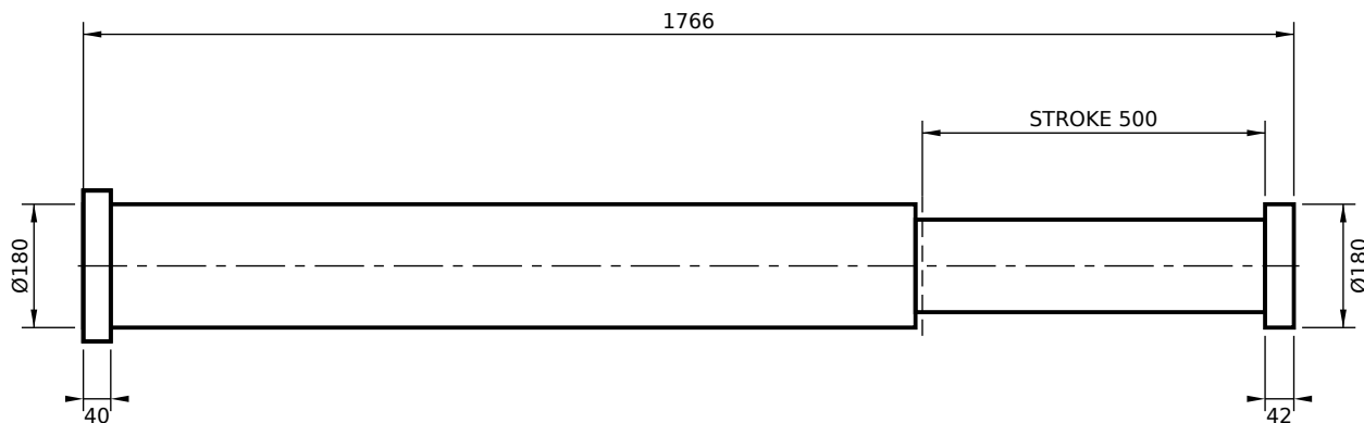
REAR FLANGE MOUNT (RS)
