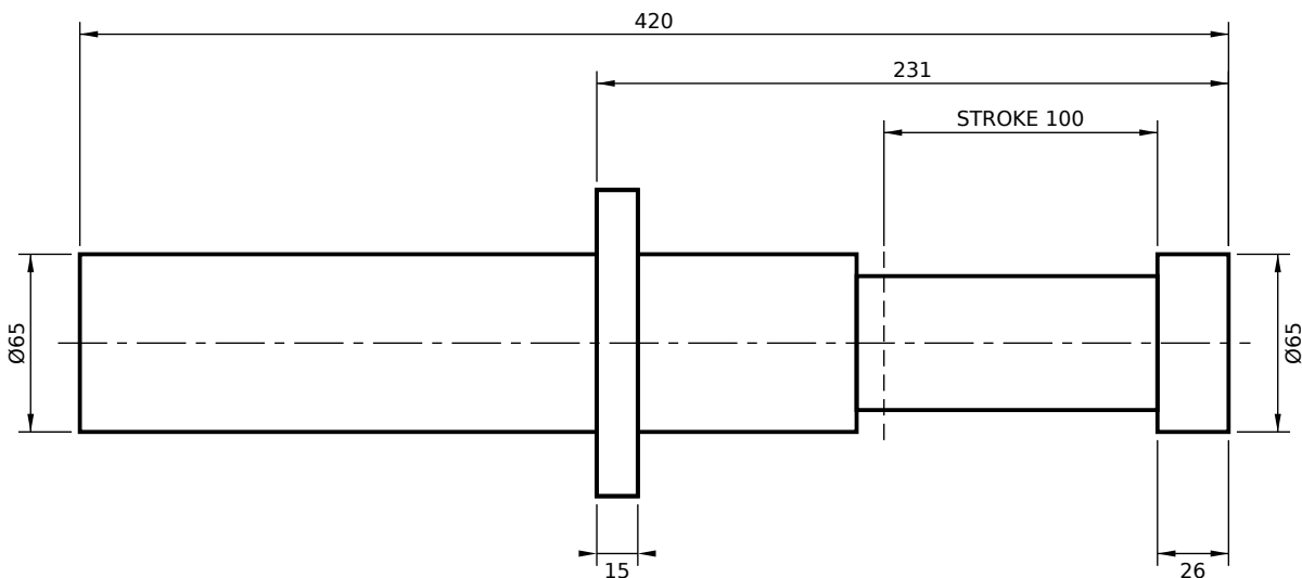
FRONT FLANGE MOUNT (FS)
