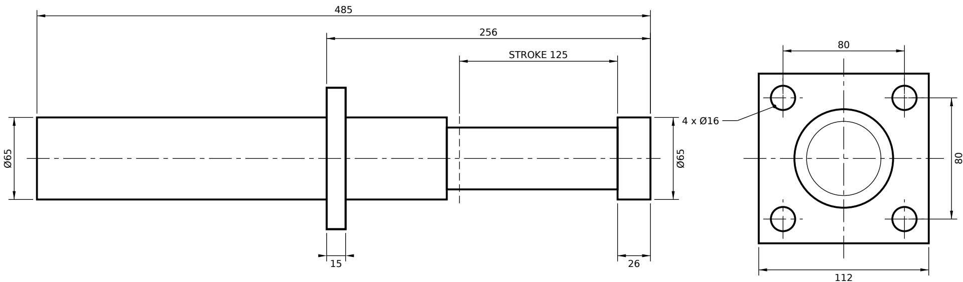
VIEW FROM ROD END (SCALE 1:2.5)
