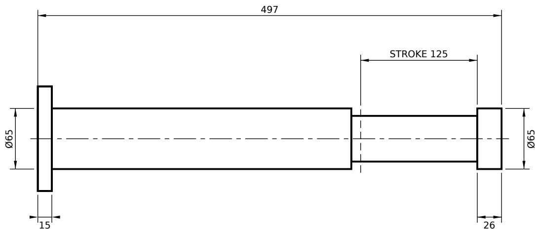
REAR FLANGE MOUNT (RS)
