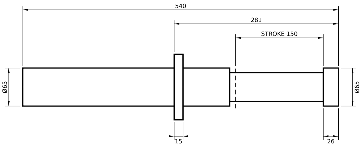
FRONT FLANGE MOUNT (FS)
