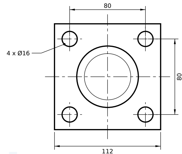
VIEW FROM ROD END
