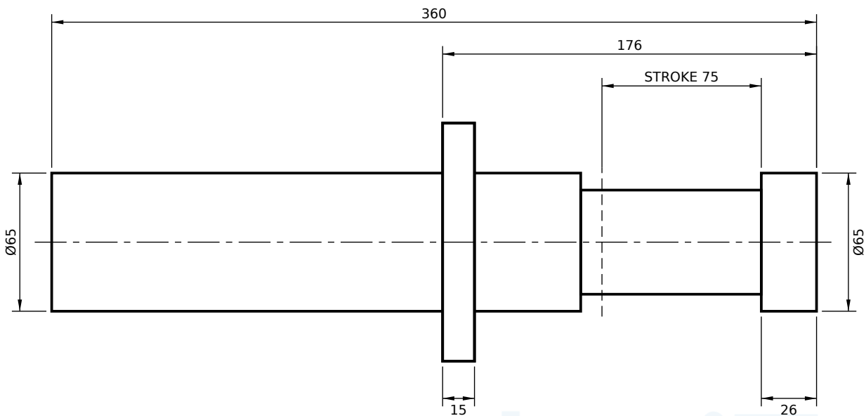
FRONT FLANGE MOUNT (FS)
