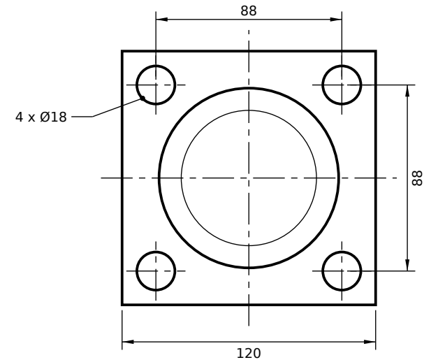
VIEW FROM ROD END (SCALE 1:2.5)
