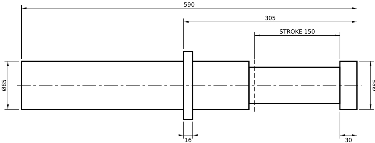
FRONT FLANGE MOUNT (FS)
