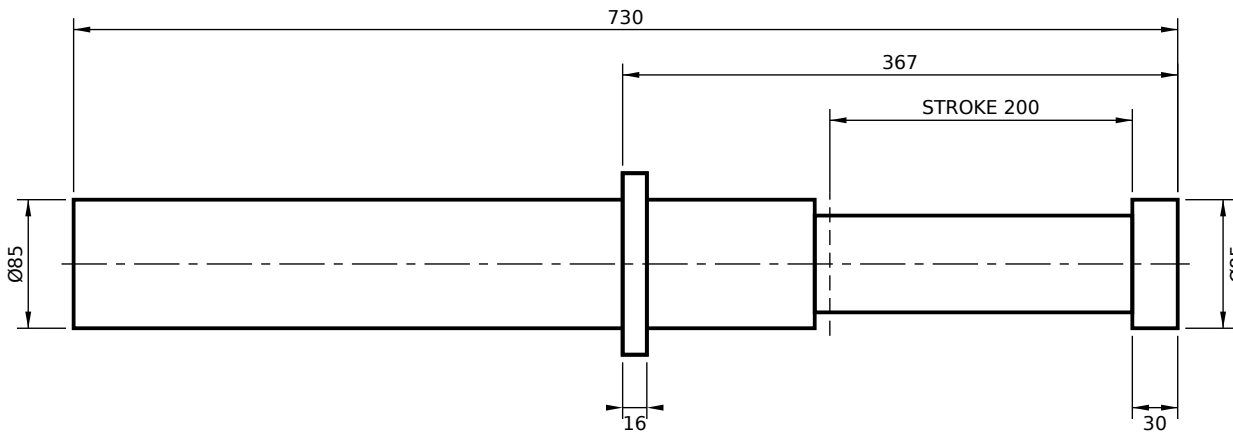
FRONT FLANGE MOUNT (FS)
